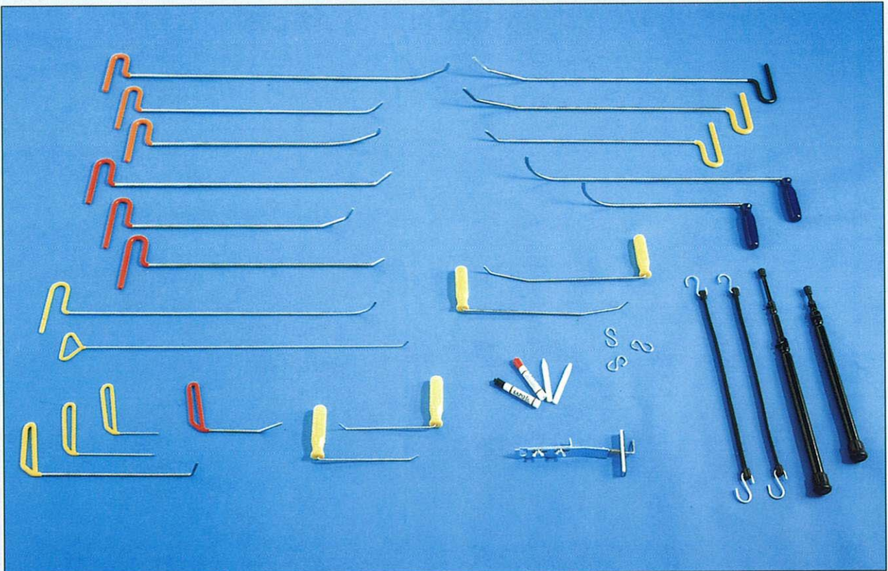
Custom kit with 21 tools (p/n 6526)
