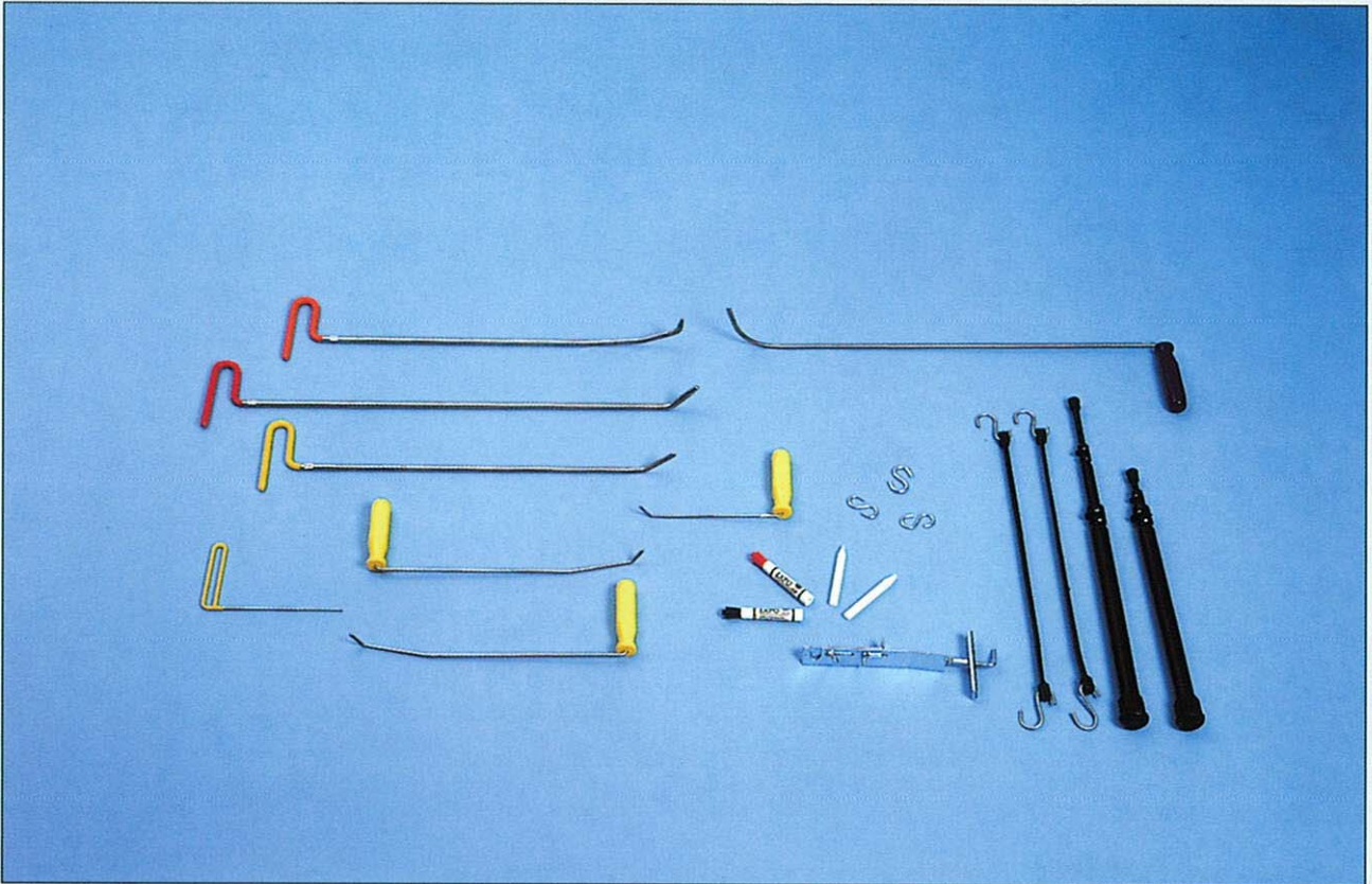
Starter kit with 8 tools (p/n 6512)
